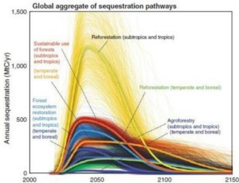
Fig. 3. Global aggregate of sequestration pathways
