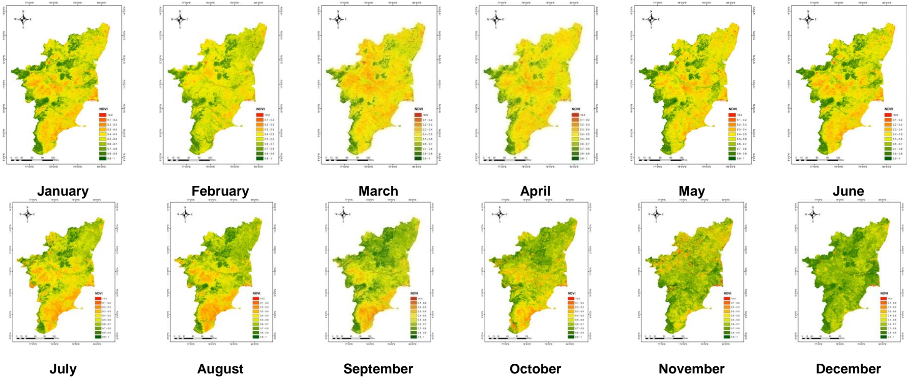
Fig. 3. MODIS NDVI product for 12 months showing crop cover phenomena for the year of 2021
