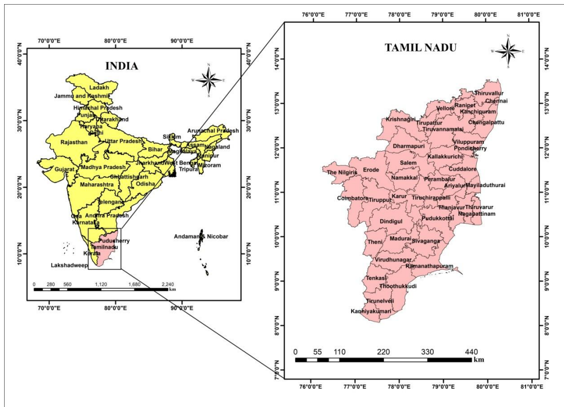
Fig. 1. Study area map – Tamil Nadu
