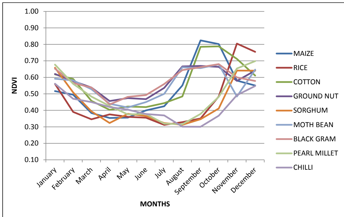
Fig. 4. Major rainfed cropping seasons of Tamil Nadu
