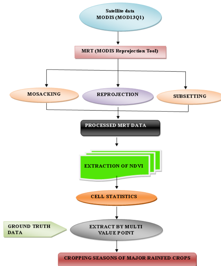
Fig. 2. Methodology for cropping season identification in major rainfed crops of Tamil Nadu
