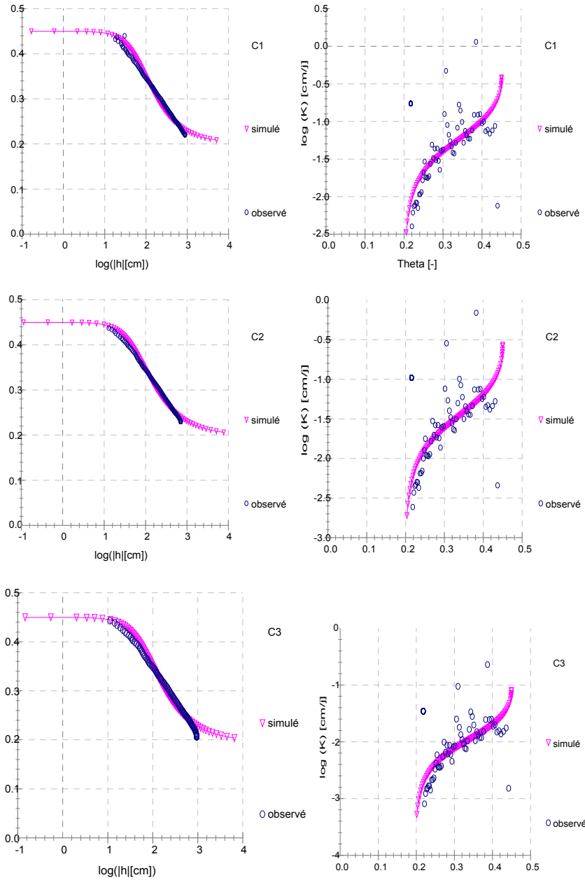
Fig. 10. h() and K() curves of the different compartments of the SSP sample
