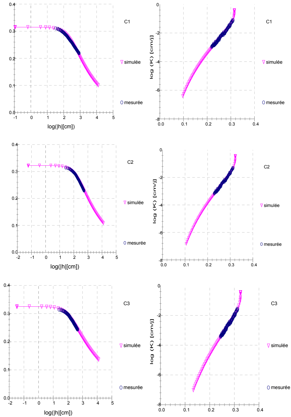
Fig. 9. h) and K) curves of the different compartments of the SSP sample fitted to the Van Genuchten - Mualem model ( m=1-1/n )
