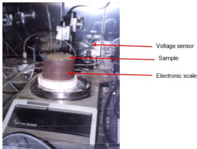
Fig. 4. View of the experimental apparatus
