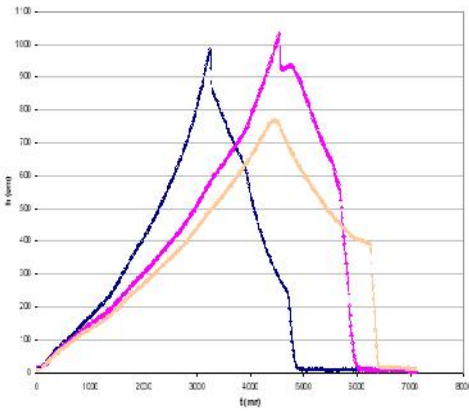
Fig. 7. SSP1-Evolution of tensiometers
