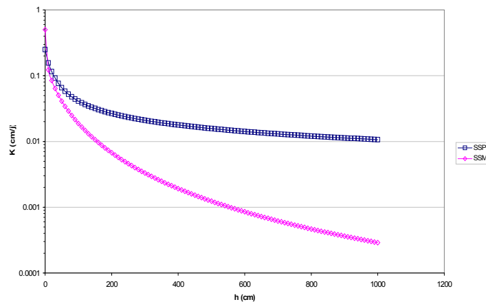
Fig. 11. Comparison of the K(h) curves of the two soils
