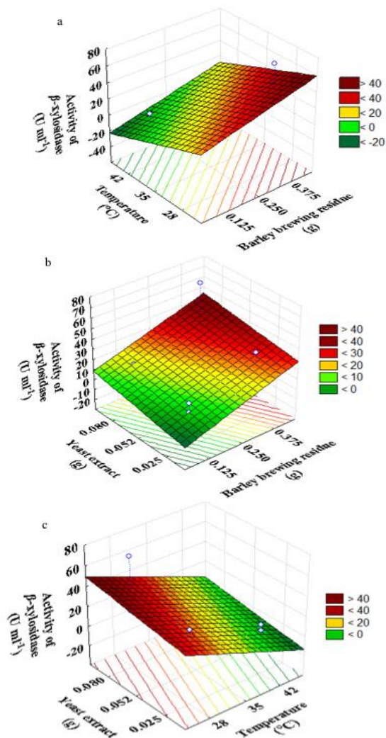
Fig. 3. (a) Response surfaces of the production of \beta -Xylosidase as functions of barley brewing residue and temperature, (b) yeast extract and barley brewing residue and (c) temperature and yeast extract, without the axial points
